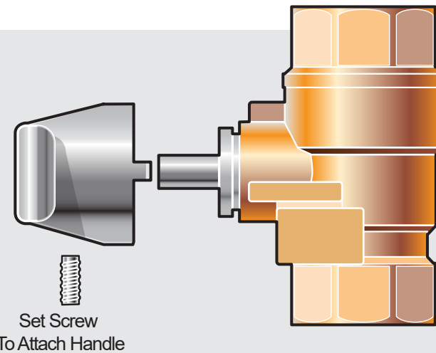
1/2" In-Line Ball Valve with with Mini Twist Handle.
