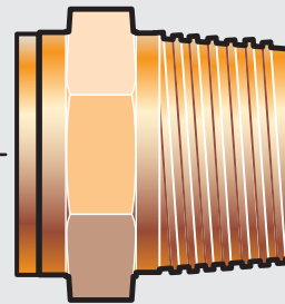
P/N 3070314 DOT Male Connector Push-in Fitting (3/4" OD Tube x 3/4" NPT)
