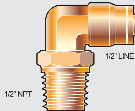
DOT Swivel Male Elbow 1/2" OD Tube x 1/2" NPT
