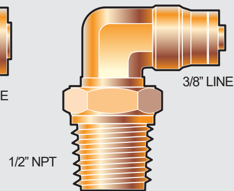
DOT Swivel Male Elbow 3/8" OD Tube x 1/2" NPT
