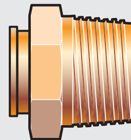
P/N 3070324 DOT Male Connector Push-in Fitting (5/8" OD Tube x 3/4" NPT)
