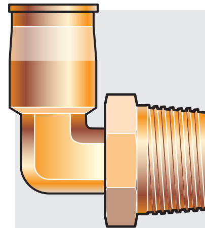
P/N 3070323 DOT Swivel Male Elbow Push-in Fitting (5/8" OD Tube x 3/4" NPT)
