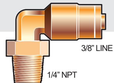
Swivel Male Elbow DOT Swivel Male Elbow 3/8" OD Tube x 1/4" NPT
