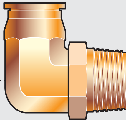
P/N 3070310 DOT Swivel Male Elbow Push-in Fitting (3/4" OD Tube x 3/4" NPT)
